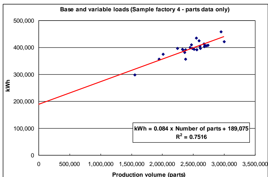
Figure 5: Base and variable loads for parts data
