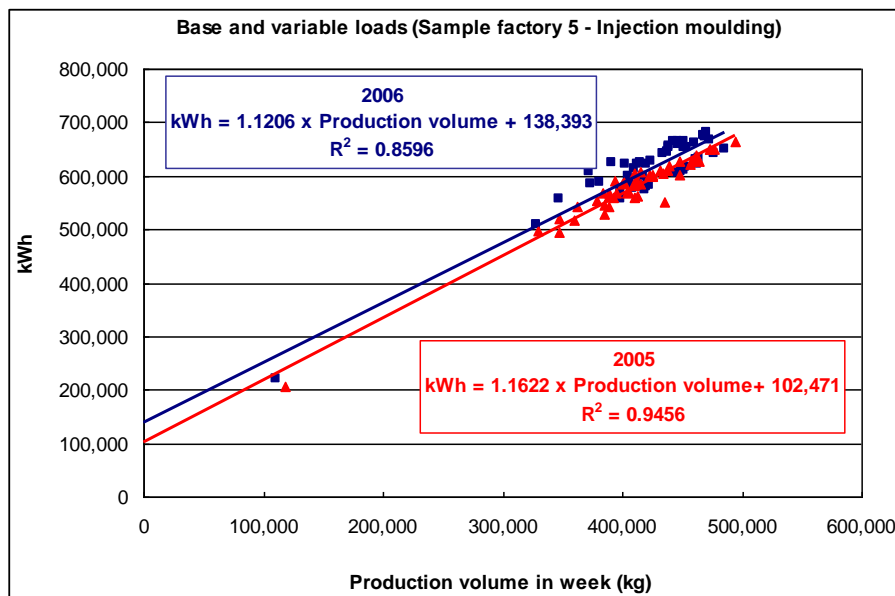
Figure 7: Comparing base and process loads after process changes
