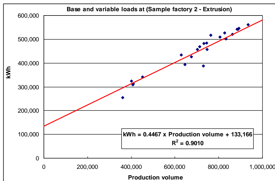
Figure 3: Base and process loads for extrusion
