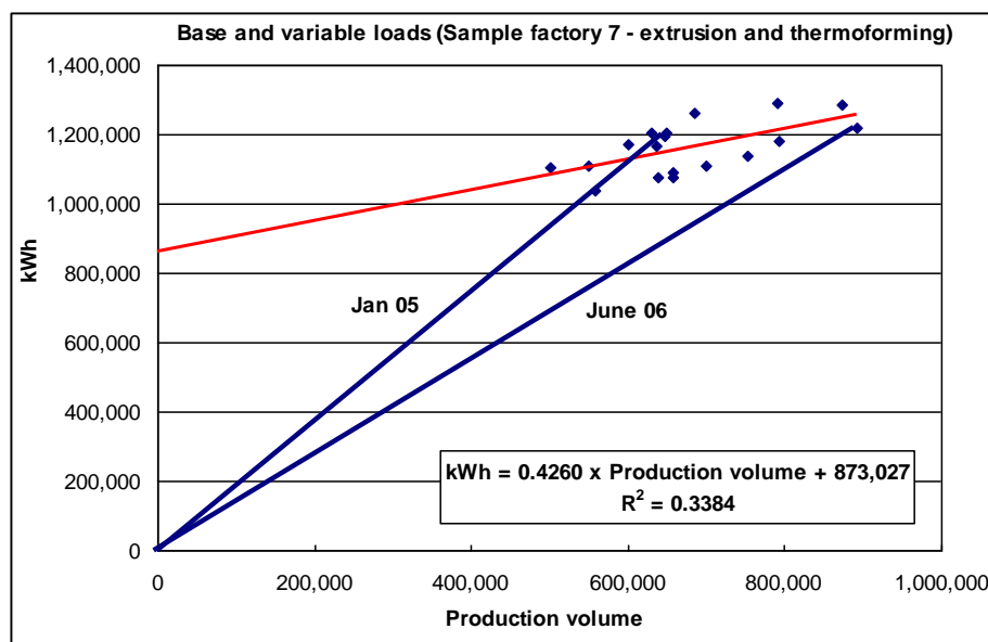
Figure 12: Simple SEC measurement
