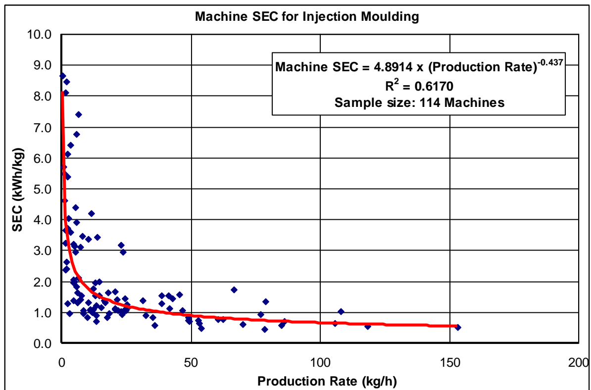
Figure 16: Machine SEC for injection moulding versus production rate
