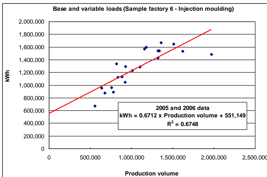
Figure 8: Comparing base and process loads after process changes
