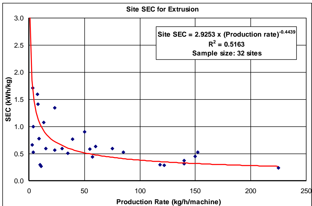
Figure 15: Site SEC for extrusion versus production rate
