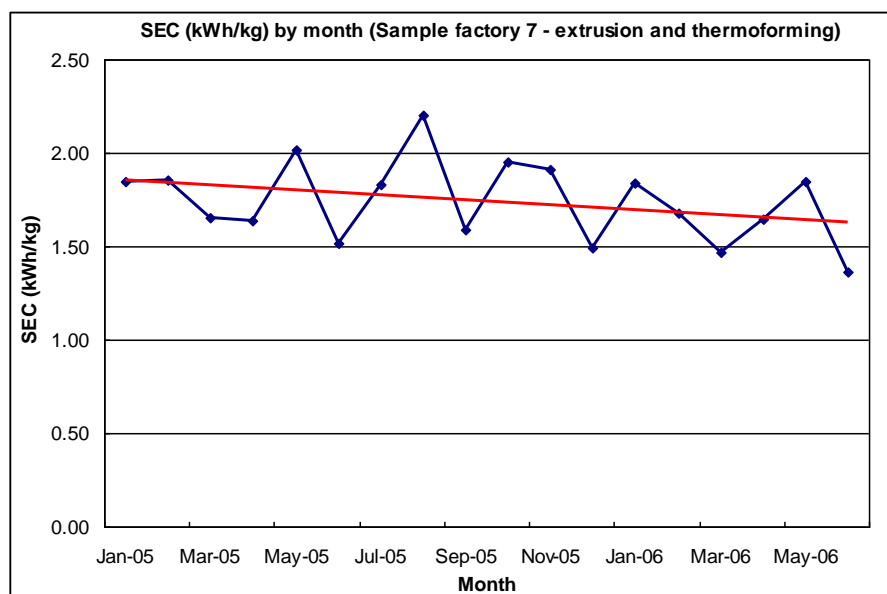
Figure 10: SEC (kWh/kg) by month
