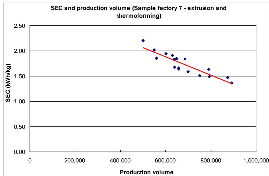
Figure 13: Production volume and SEC
