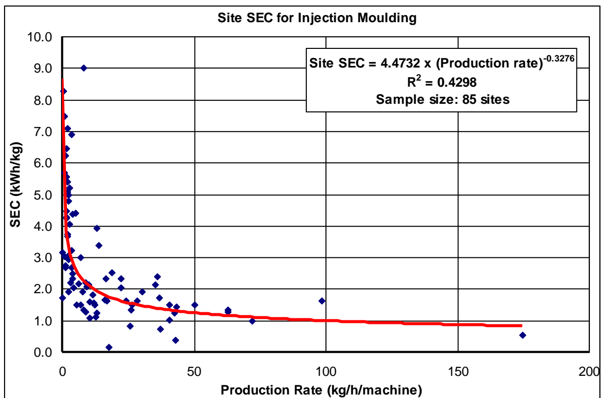
Figure 14: Site SEC for injection moulding versus production rate
