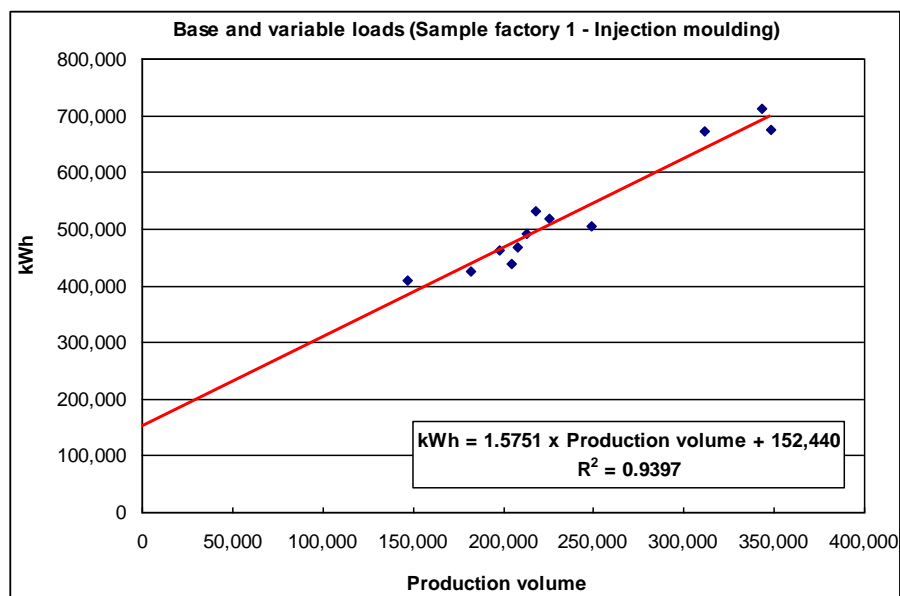
Figure 2: Determining the base and process loads
