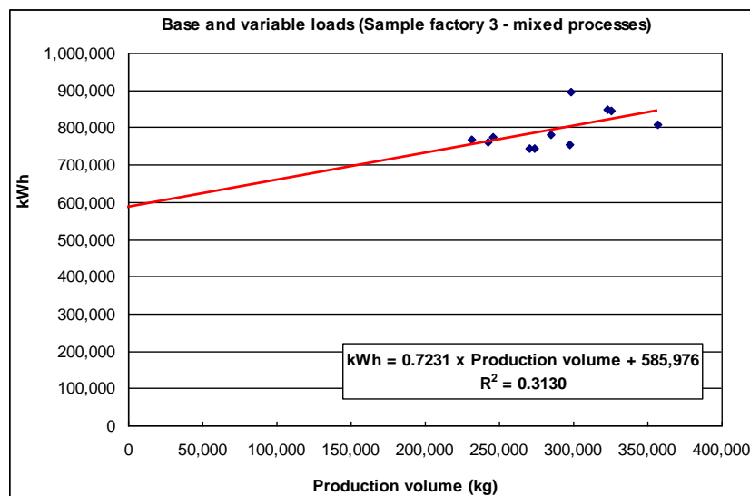
Figure 4: Base and variable loads for mixed processing
