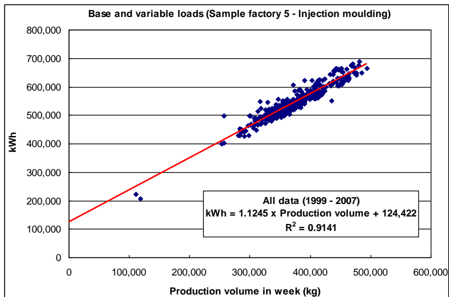
Figure 6: Base and process loads over the long term (8 years of weekly data)
