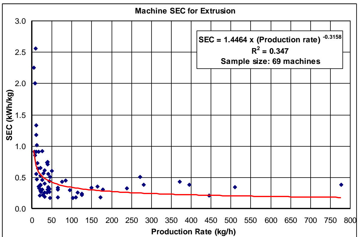
Figure 17: Machine SEC for extrusion versus production rate
