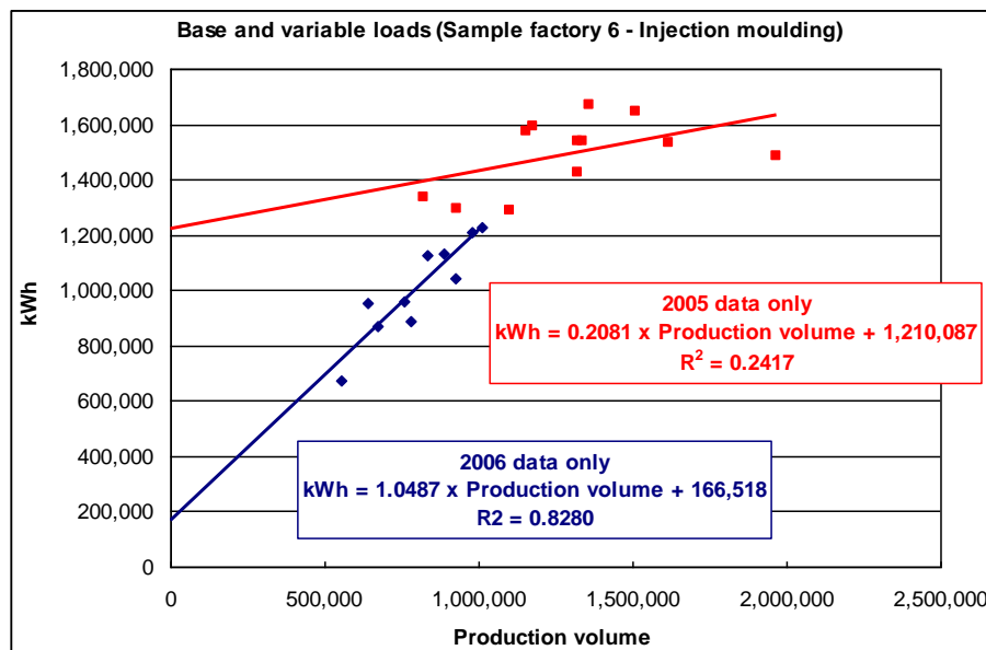
Figure 9: Comparing base and process loads after management changes
